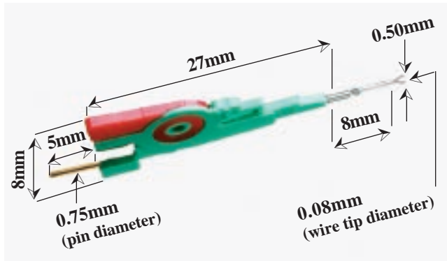
0.5mm to 0.3mm MicroGripper
